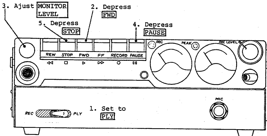
Fig. 3 Playback Procedure
